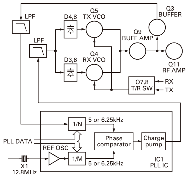
Fig. 5 PLL circuit
